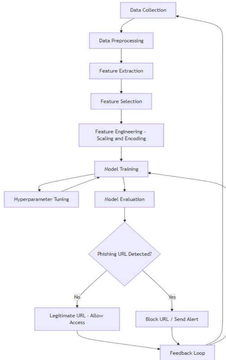
Fig 1: Flowchart of the Proposed Phishing URL Detection System
